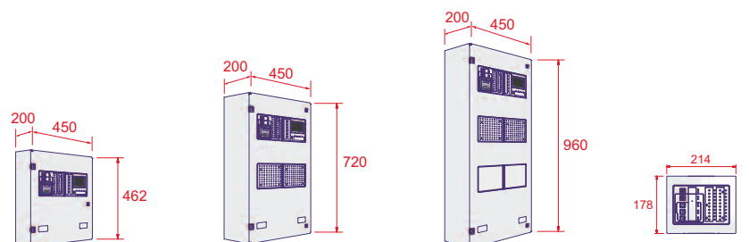
Standard (1-4 loop) (18Ah Batteries) Medium (2-4-6-8 loop) (12-38Ah Batteries) Large (2-4-6-8 loop) (12-38Ah Batteries) Compact Controller
